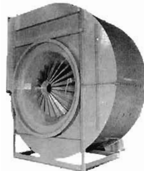
Arrangement 1, SWSI, Class III fan with rigidly braced housing. split for ease of wheel removal and inlet vane control.
