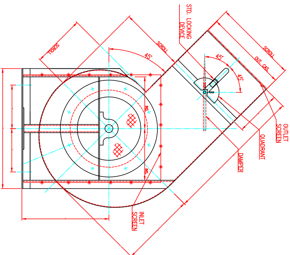
INLET SIDE ELEVATION
